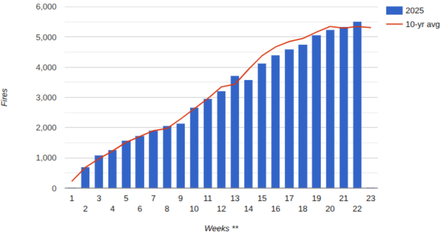
Seasonal fire occurrence
